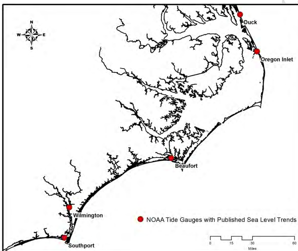
Figure 6. Location of NOAA tide gauges with published sea level trends in North Carolina.
