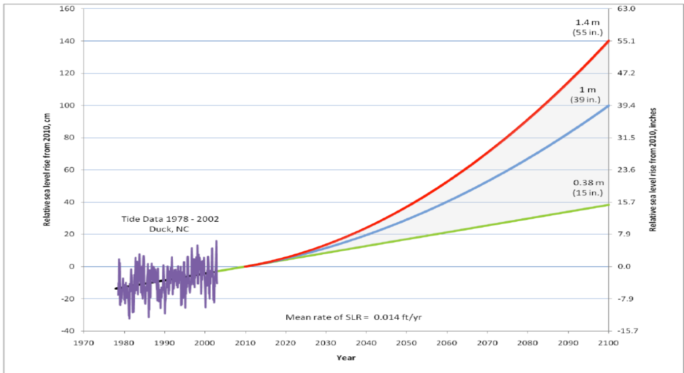
Figure 2. This chart illustrates the magnitude of SLR resulting from differing rates of acceleration. The most likely scenario for 2100 AD is a rise of 0.4 meter to 1.4 meters (15 inches to 55 inches) above present.
